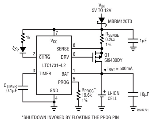
Figure 1. Single Cell 500mA Li-Ion Battery Charger
