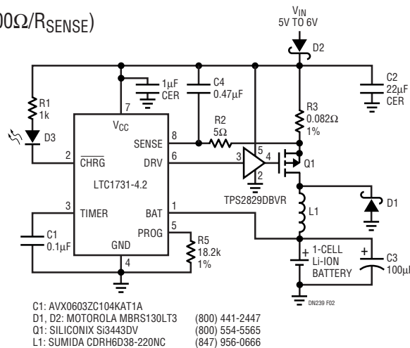
Figure 2. Single Cell 1.5A Li-Ion Battery Charger
